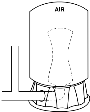
WATER CELL IS COMPLETELY EMPTY: A new cycle is ready to begin. Simple, positive action produces maximum drawdown on every cycle.
