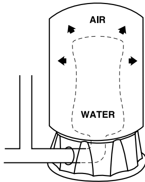
WATER BEGINS TO ENTER THE TANK: Air is compressed around the water cell as it fills with water.
